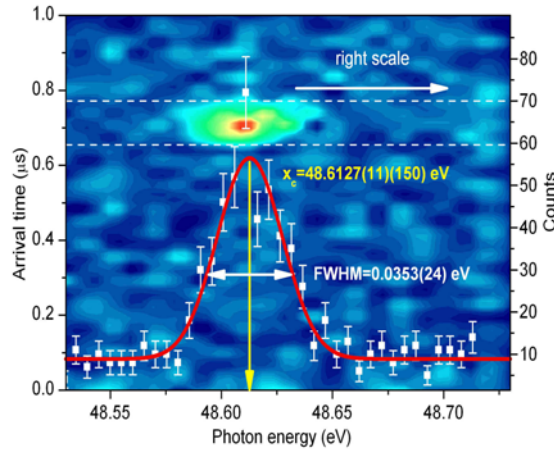
Fig. 2: 2D plot of the fluorescence signal as a function of the photon arrival time relative to the FLASH pulse (left y-axis, arbitrary offset) versus photon energy (x-axis) after 1987 s (smoothed data, 5 \text{ meV} \times 0.016 \text{ } \mu\text{s} binning). Inset: Projection of the relevant band (white lines; white squares) onto the photon energy axis yielding the number of photons (right y-axis) as a function of their energy. Red line: Gaussian fit.
